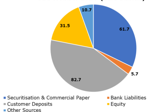
VWFS Funding Structure as at 31 December 2024 (Euro Billions)
