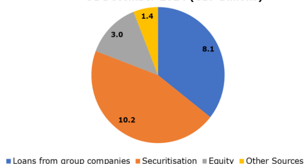
VWFS (UK) Funding Structure as at 31 December 2024 (GBP Billions)
